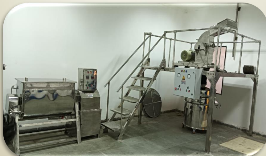
SPICES PROCESSING & GRINDING LINE
